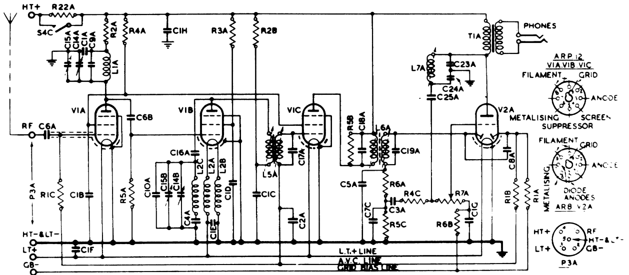
Schema 2 (Ontvanger).
